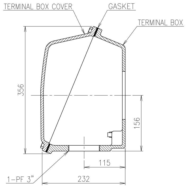
SEC. A-A'
