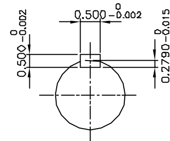
OUTPUT SHAFT
