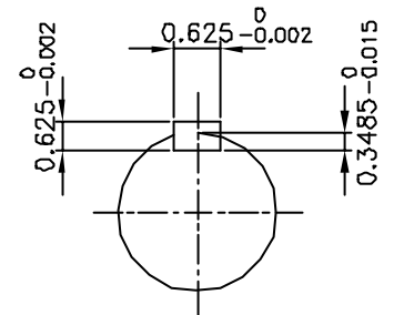
OUTPUT SHAFT
