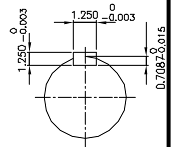
OUTPUT SHAFT
