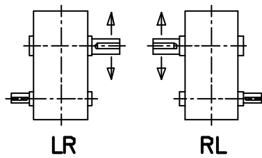
LR RL SHAFT ARRANGEMENT & DIRECTION of ROTATION
