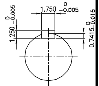
OUTPUT SHAFT
