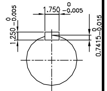
OUTPUT SHAFT
