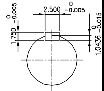
OUTPUT SHAFT
