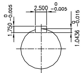
OUTPUT SHAFT
