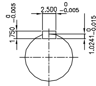
OUTPUT SHAFT
