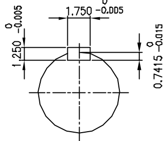
OUTPUT SHAFT
