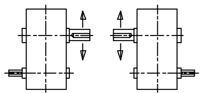
SHAFT ARRANGEMENT & DIRECTION of ROTATION
