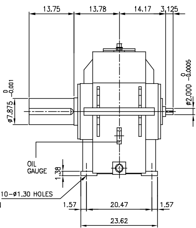
OUTPUT SHAFT
