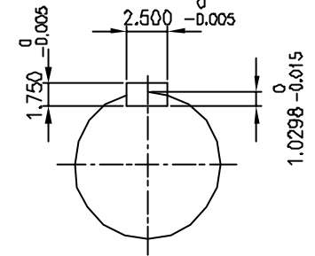
OUTPUT SHAFT
