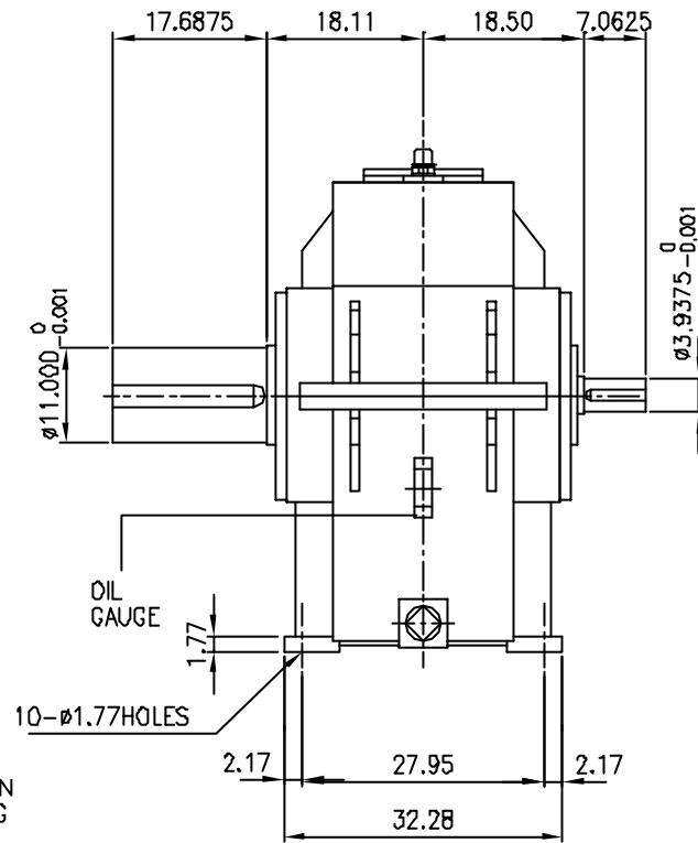
OUTPUT SHAFT
