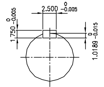
OUTPUT SHAFT
