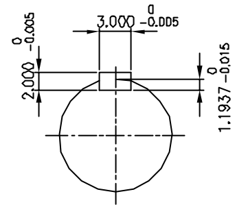
OUTPUT SHAFT
