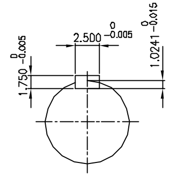
OUTPUT SHAFT
