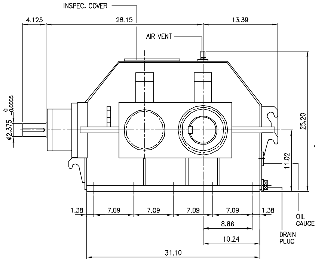
OUTPUT SHAFT
