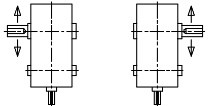
SHAFT ARRANGEMENT & DIRECTION of ROTATION
