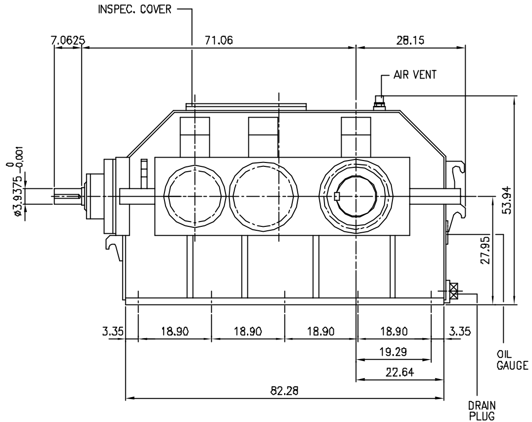
OUTPUT SHAFT
