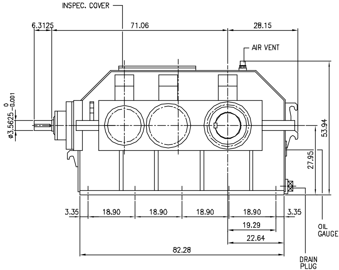
OUTPUT SHAFT
