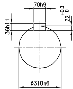
OUTPUT SHAFT
