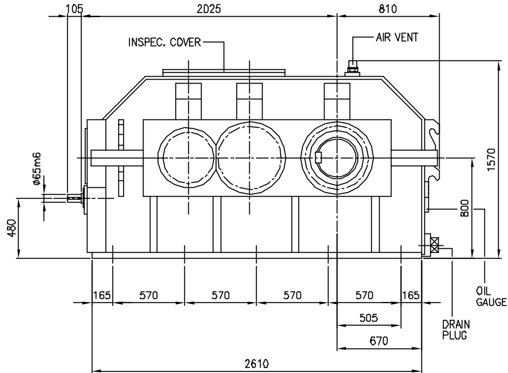
OUTPUT SHAFT
