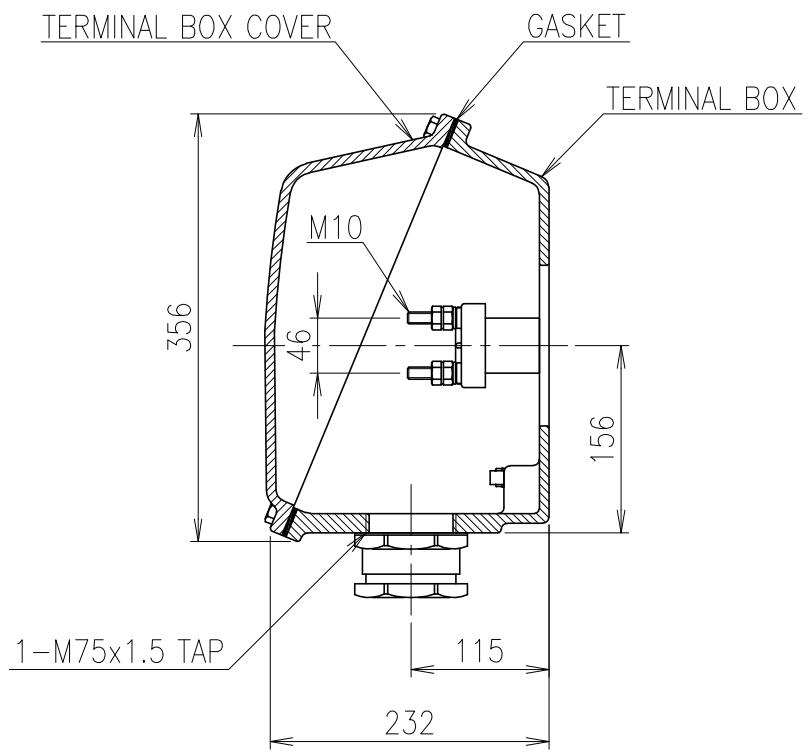
SEC. A-A'
