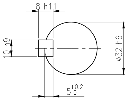
OUTPUT SHAFT KEY 10 x 8 x 48
