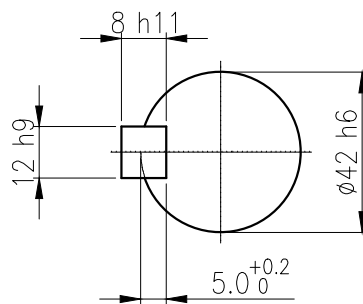
OUTPUT SHAFT
