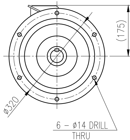
VIEW "Q"
