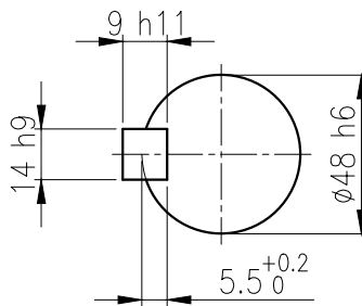
OUTPUT SHAFT
