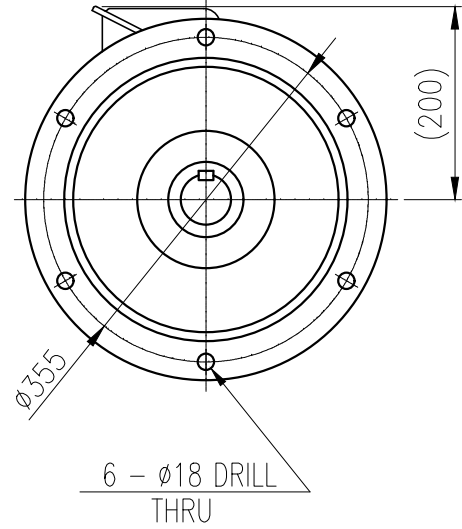
VIEW "Q"
